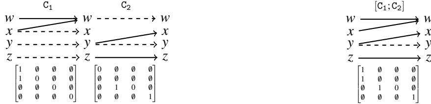
Figure 7: Composition of independent chunks of commands
