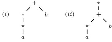
■ Figure 5 Example of two trees of size n = 5 , for regular expressions, having different probabilities for any choice of distribution. The probability of the trees in (i) and (ii) are \frac{1}{3}p_+p_*p_ap_b and \frac{1}{2}p_+p_*p_ap_b respectively.
