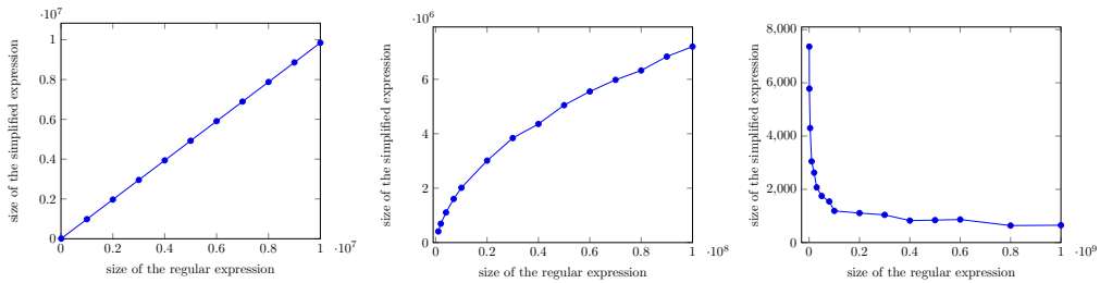
■ Figure 4 The three main regimes observed experimentally on regular expressions on two letters, with 10 000 samples for each size: (from left to right) linear ( p_+ = p_{\star} = p = 1/3 ), sublinear ( p_+ = 19/29, p_{\star} = p = 5/29 ) and constant ( p_+ = 8/10, p_{\star} = p = 1/10 ).
