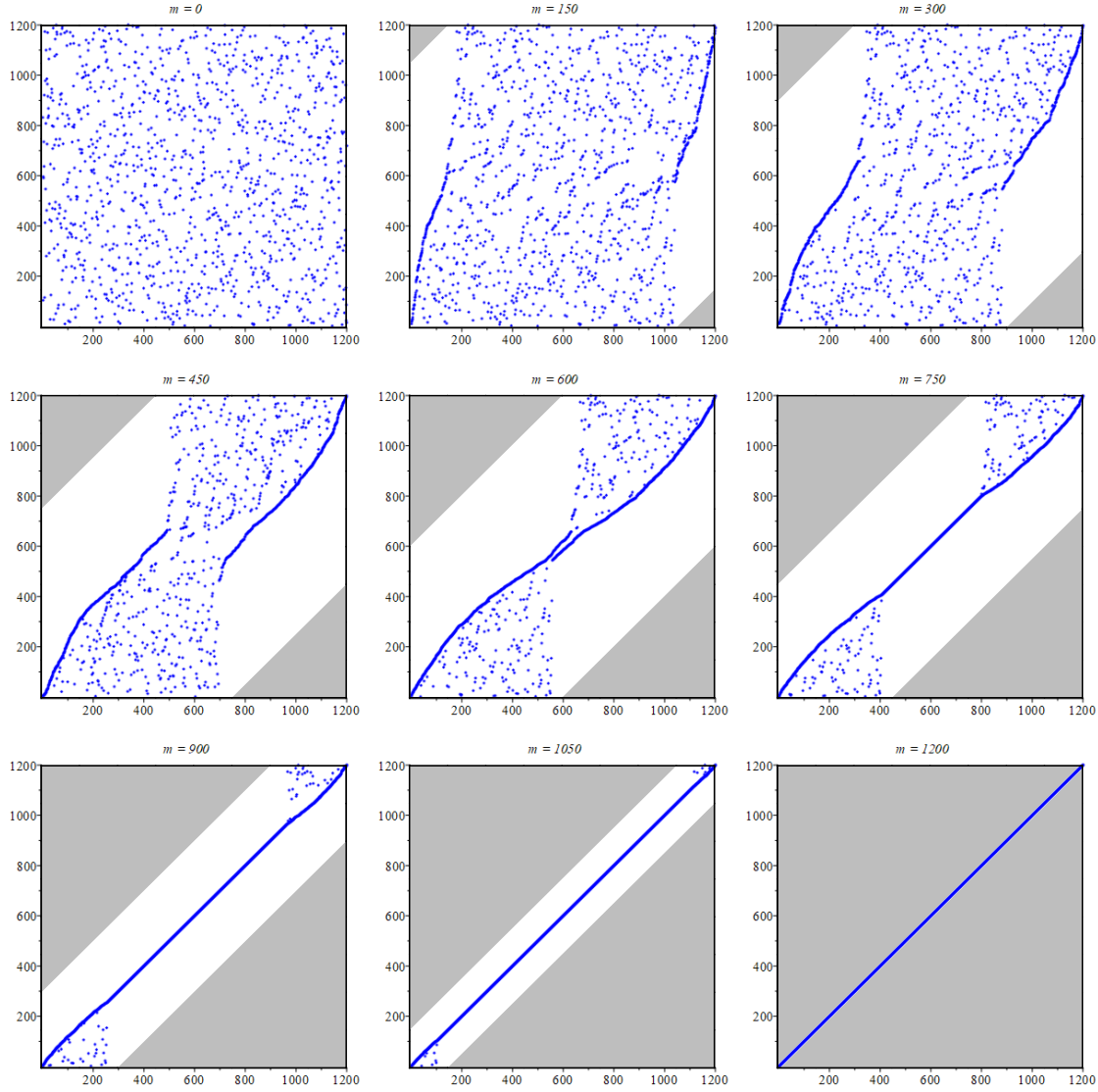
Fig. 3: The evolution of the flip-sort algorithm on a sample permutation of size n = 1200 . In this article, we show that for any input permutation, there are two areas (the grey areas in the above plots, which are proportional to the number m of iterations) without any dots inside. This entails that the permutations “shrink” (in the white area) until they finally get fully sorted (after \leq n - 1 iterations). We also show that, for all m , for any coordinates in the white area, there exists an input permutation which will have a dot at these coordinates. (See lipn.fr/~cb/Papers/popstack.html for some animations of this flip-sort process.)
