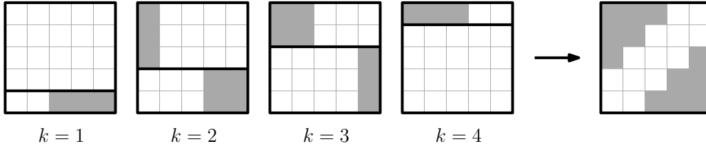
Fig. 16: Illustration to proof of Theorem 21 for n = 5 : forbidden areas for fixed m ( m = 3 ).
